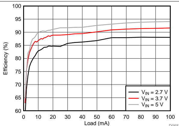
Figure 76. LCM Boost Efficiency
