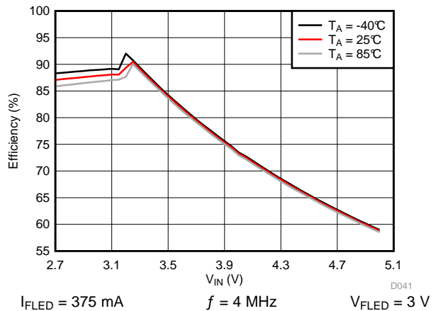
Figure 115. Torch System Efficiency
